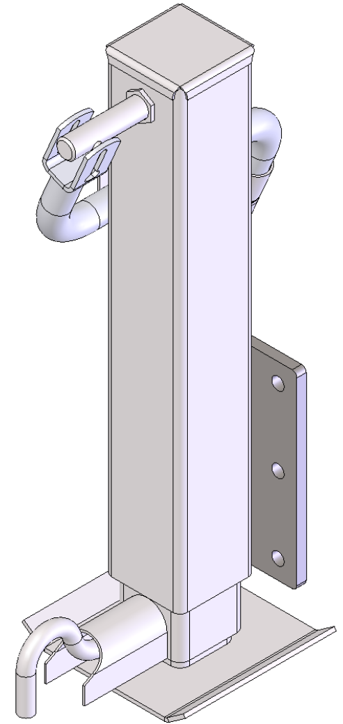
J04044 FRONT JACKSTAND
