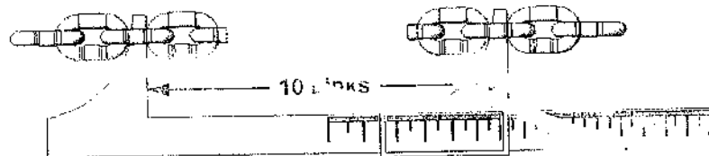
Figure 10 - Chain Inspection
