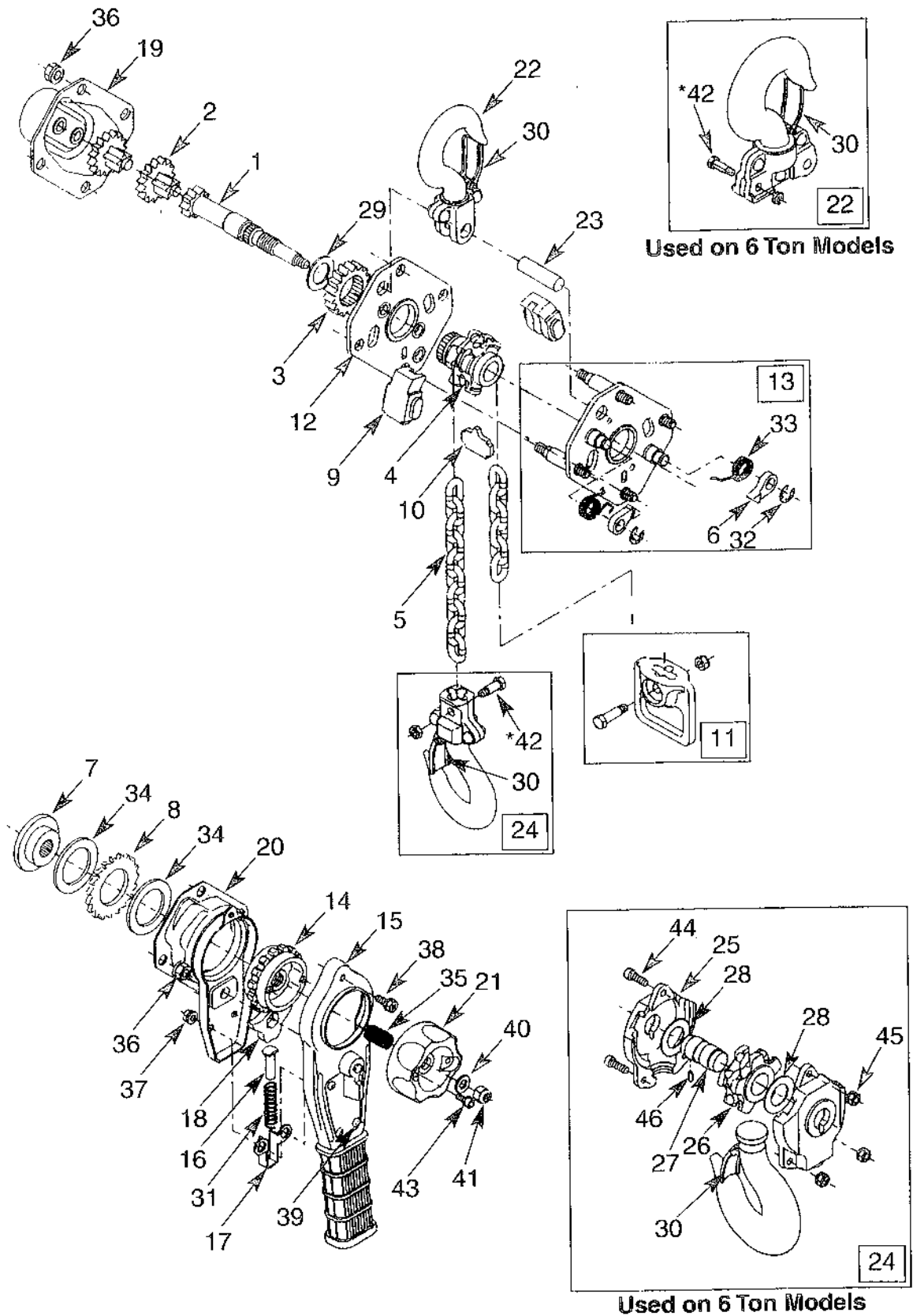
Figure 16 - 3 & 6 Ton Models
