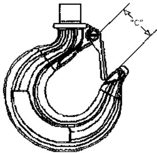
Figure 11 - Hook Inspection
