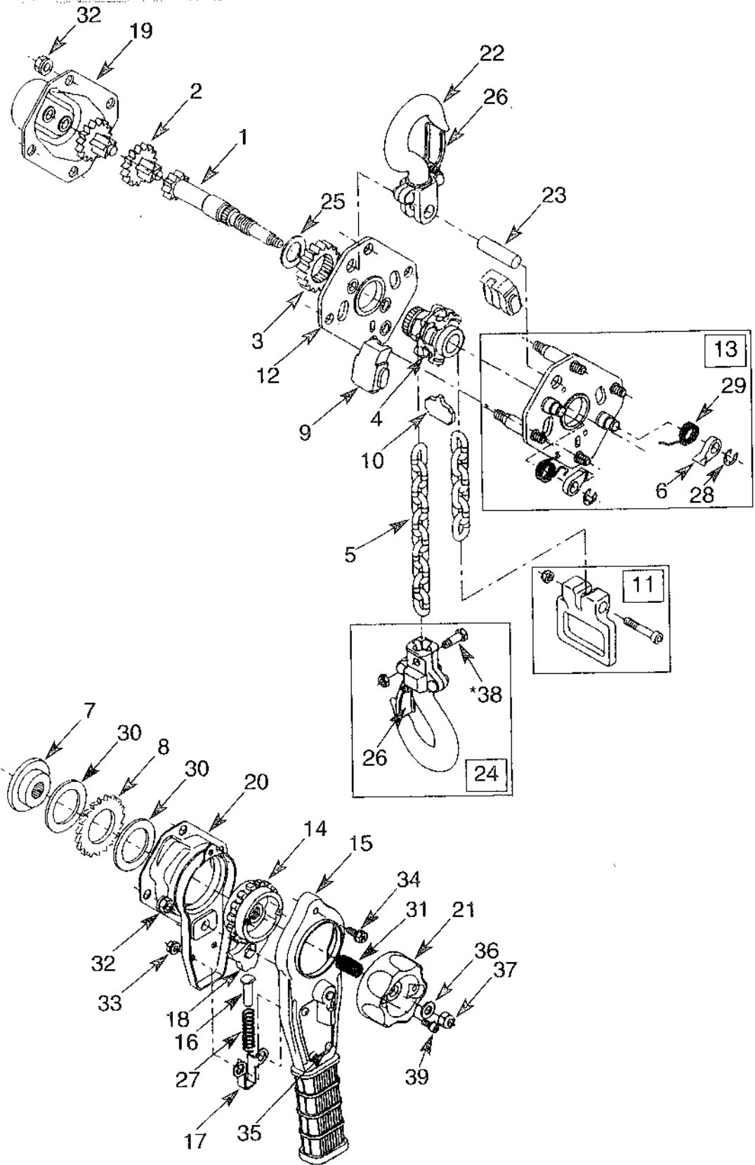
Figure 15 - .75, 1.0 & 1.5 Ton Models
